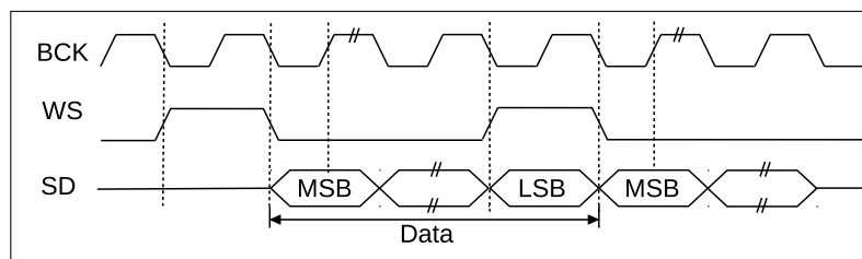
Figure 63: PCM Standard
