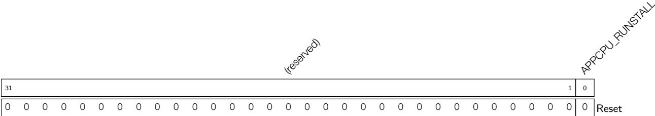
Register 5.7: APPCPU_CTRL_REG_C_REG (0x034)
