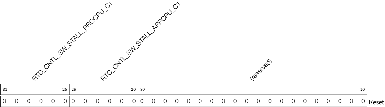
Register 30.32: RTC_CNTL_SW_CPU_STALL_REG (0x002b)
