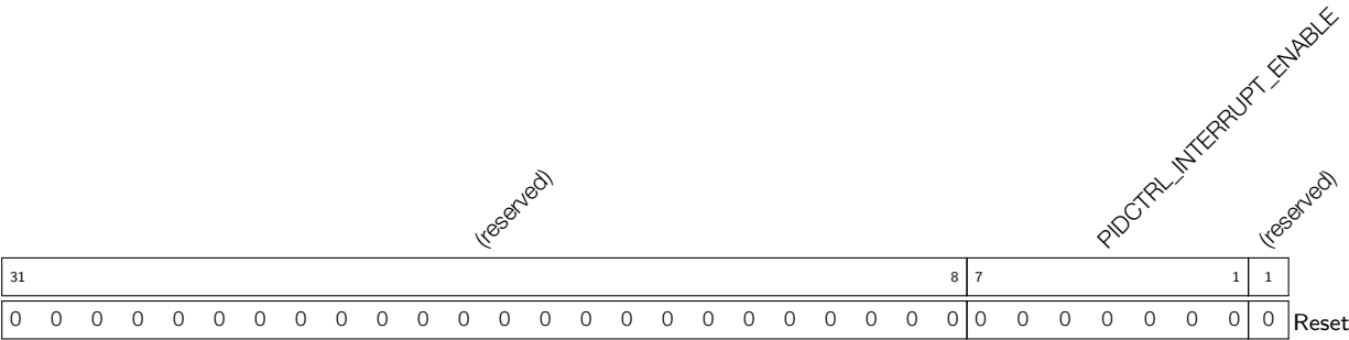
Register 27.1: PIDCTRL_INTERRUPT_ENABLE_REG (0x000)
