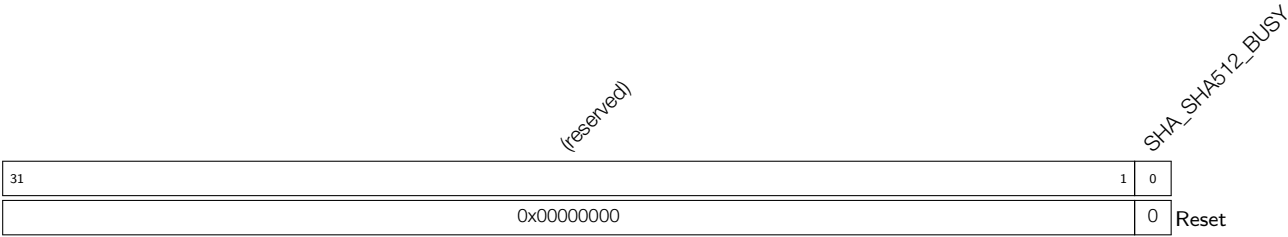
Register 22.17: SHA_SHA512_BUSY_REG (0x0BC)
