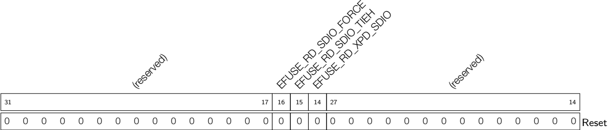
Register 20.5: EFUSE_BLK0_RDATA4_REG (0x010)
