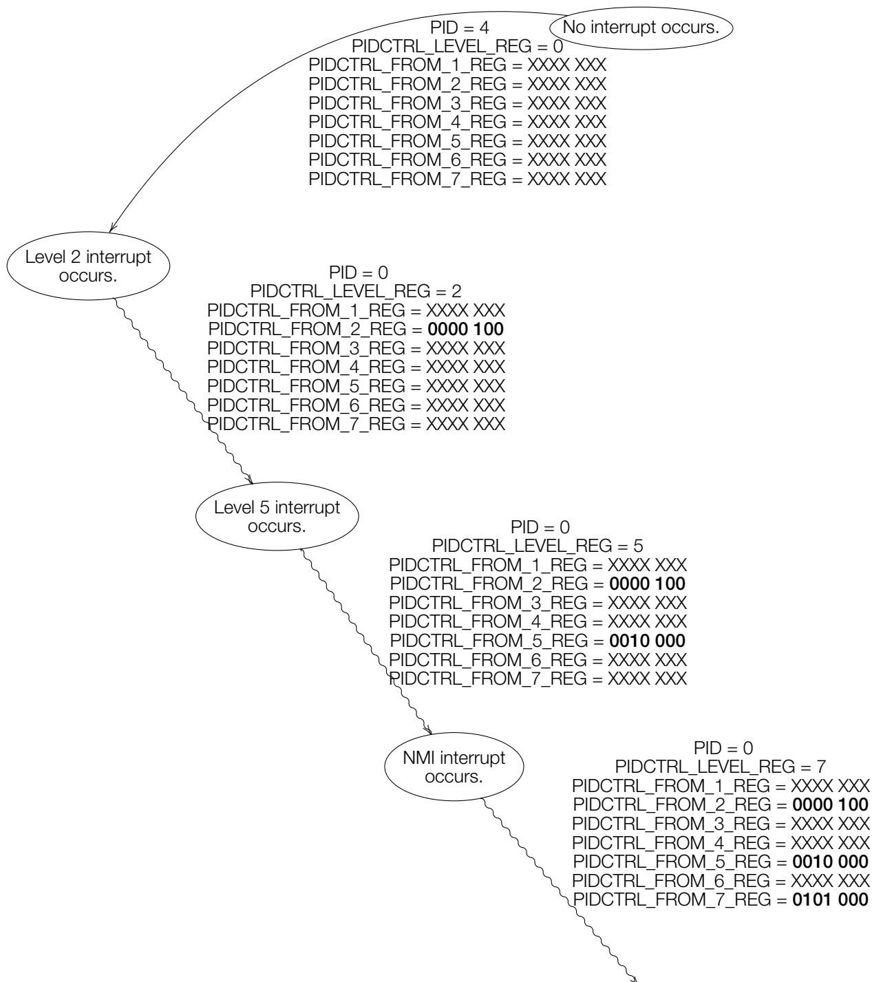
Figure 124: Interrupt Nesting
