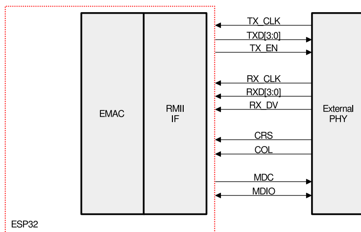
Figure 41: MII Interface
