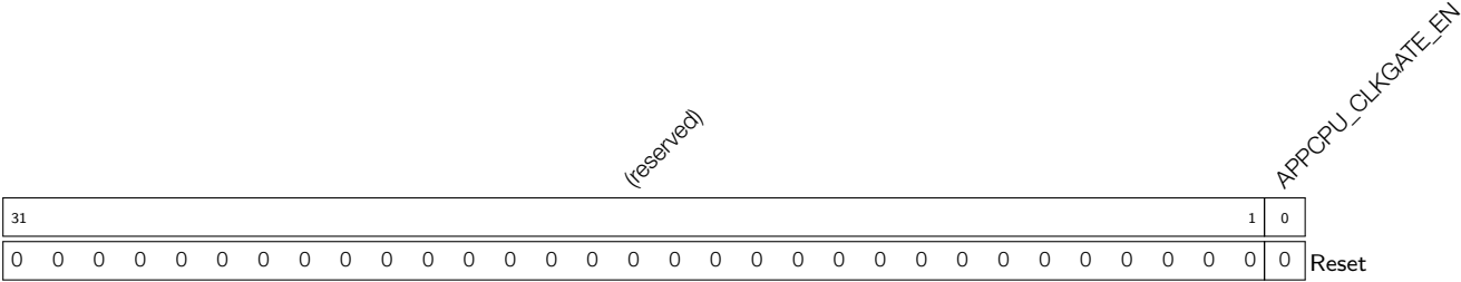
Register 5.6: APPCPU_CTRL_REG_B_REG (0x030)
