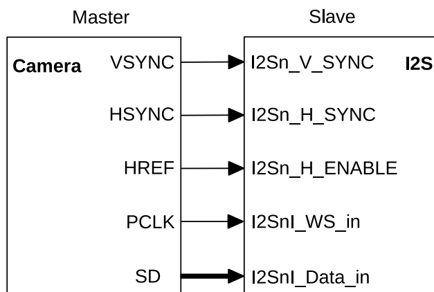
Figure 74: Camera Slave Receiving Mode
