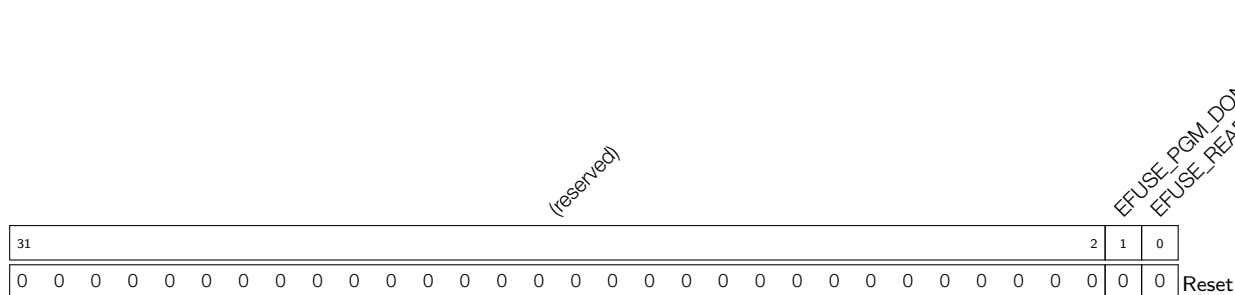
Register 20.25: EFUSE_INT_ST_REG (0x10c)
