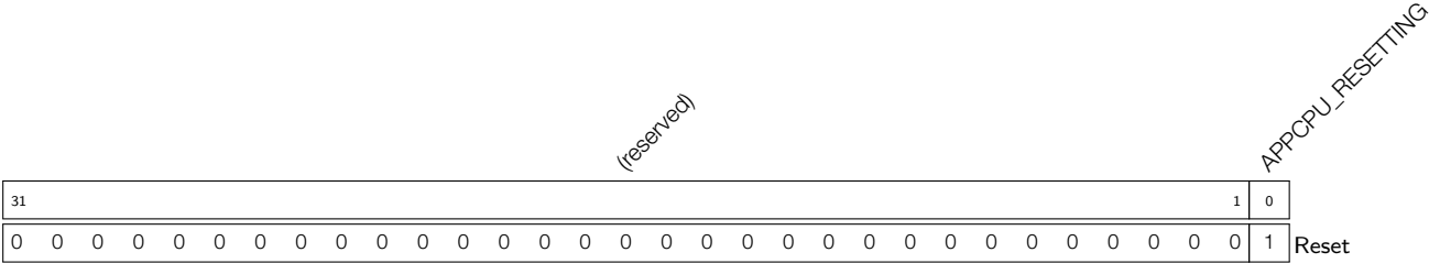
Register 5.5: APPCPU_CTRL_REG_A_REG (0x02C)
