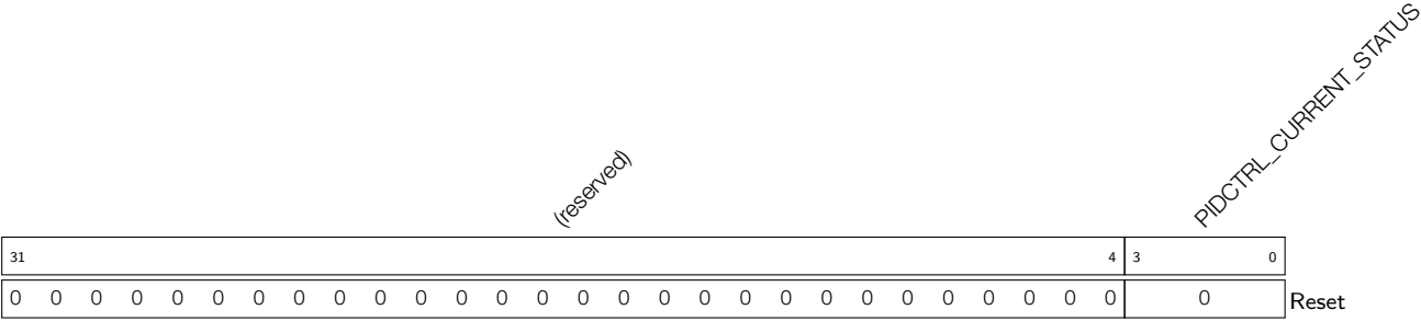
Register 27.11: PIDCTRL_LEVEL_REG (0x028)
