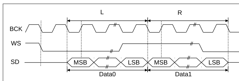
Figure 61: Philips Standard
