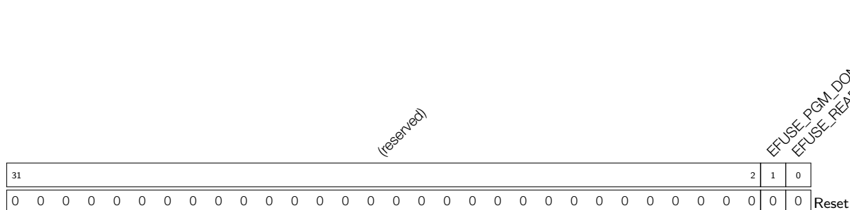
Register 20.26: EFUSE_INT_ENA_REG (0x110)
