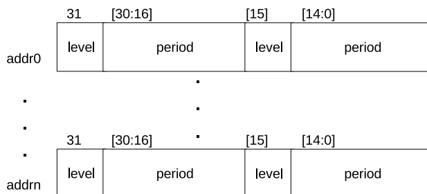
Figure 89: Data Structure
