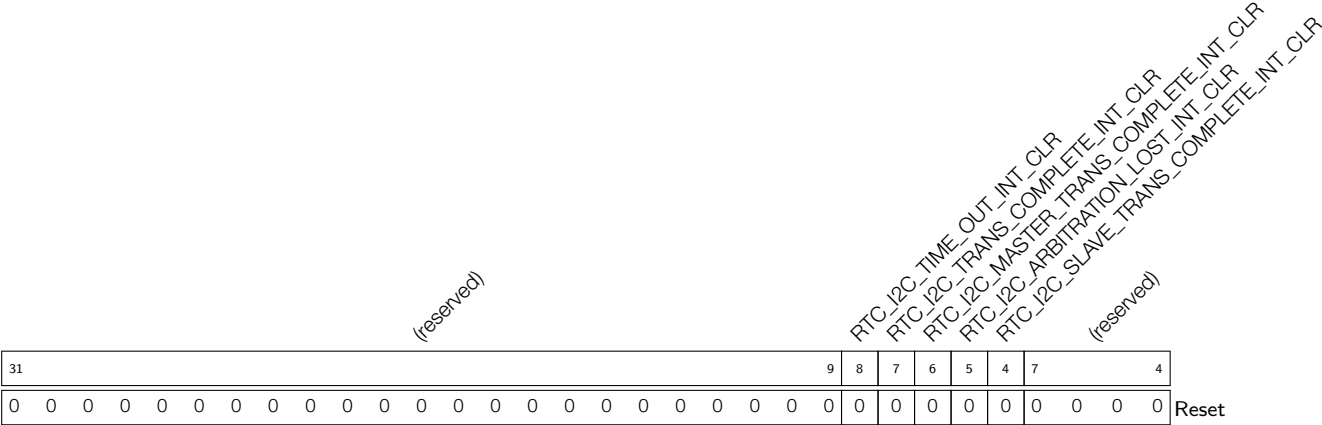
Register 29.13: RTC_I2C_INT_CLR_REG (0x024)
