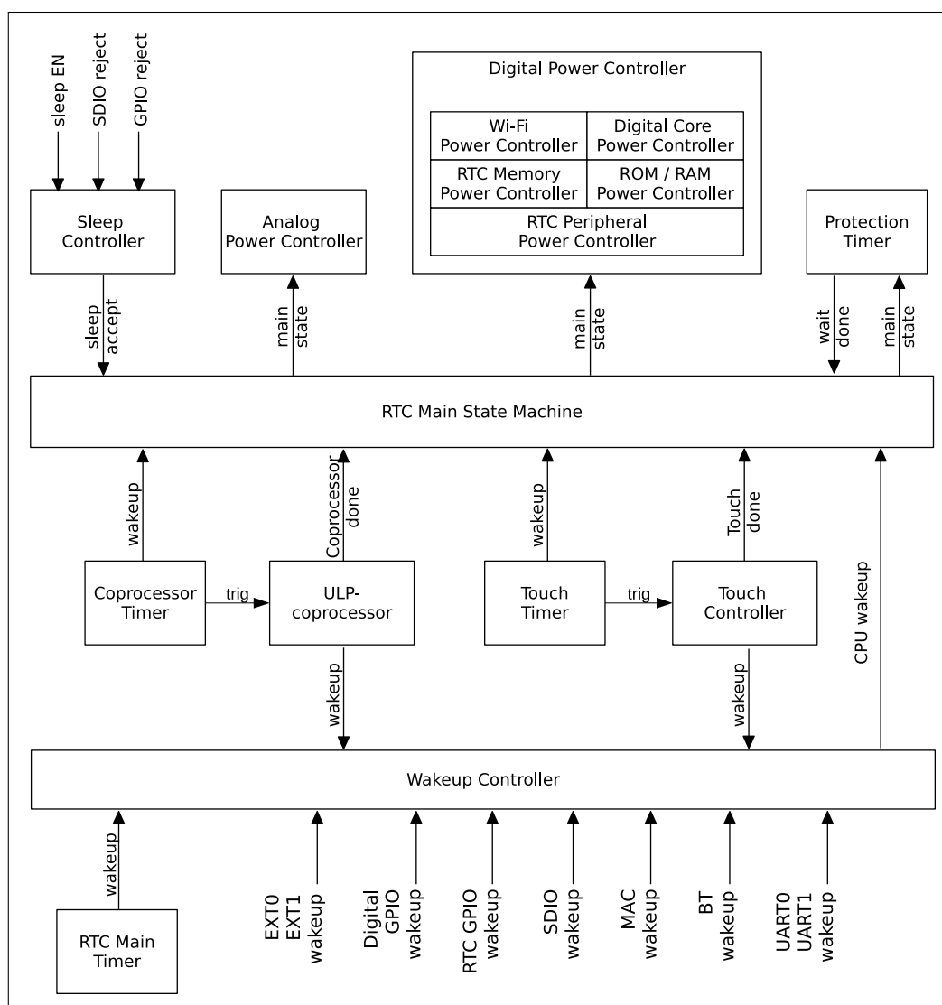
Figure 167: RTC Structure
