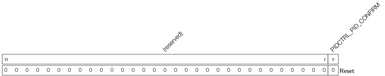
Register 27.14: PIDCTRL_PID_CONFIRM_REG (0x04C)
