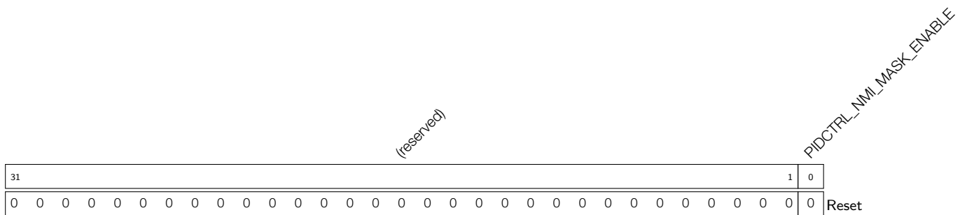
Register 27.15: PIDCTRL_NMI_MASK_ENABLE_REG (0x054)
