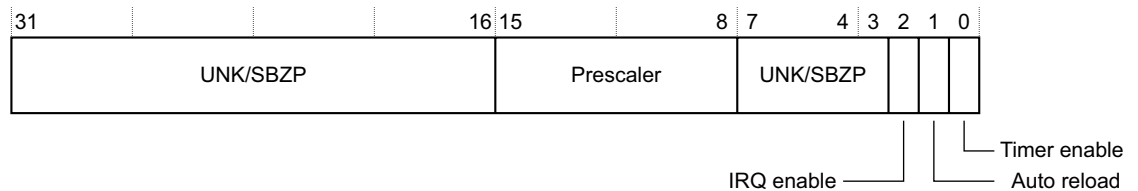
Figure 4-1 Private Timer Control Register bit assignments
